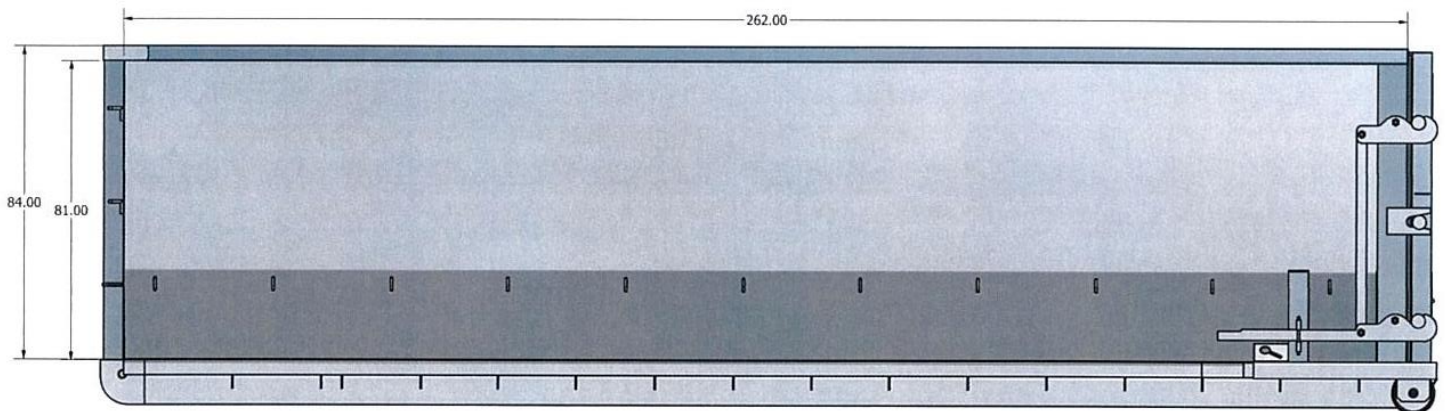
LATCH SIDE VIEW
